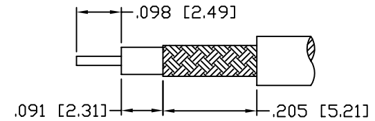
RECOMMENDED STRIPPING DIMENSIONS
