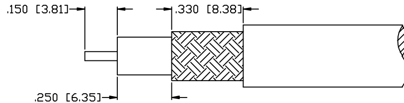
RECOMMENDED STRIPPING DIMENSIONS
