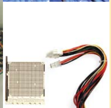
Power Cables
